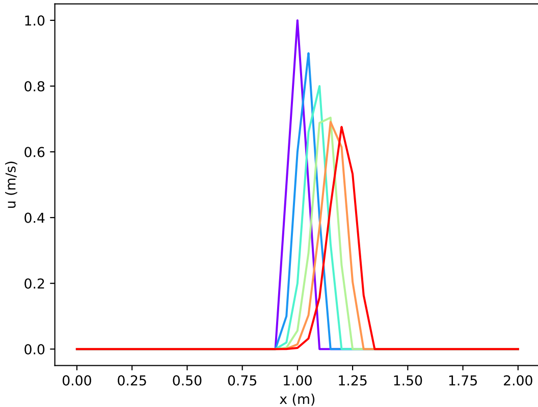
Figure 1: \sigma=0.8 , Backward Differencing in x
