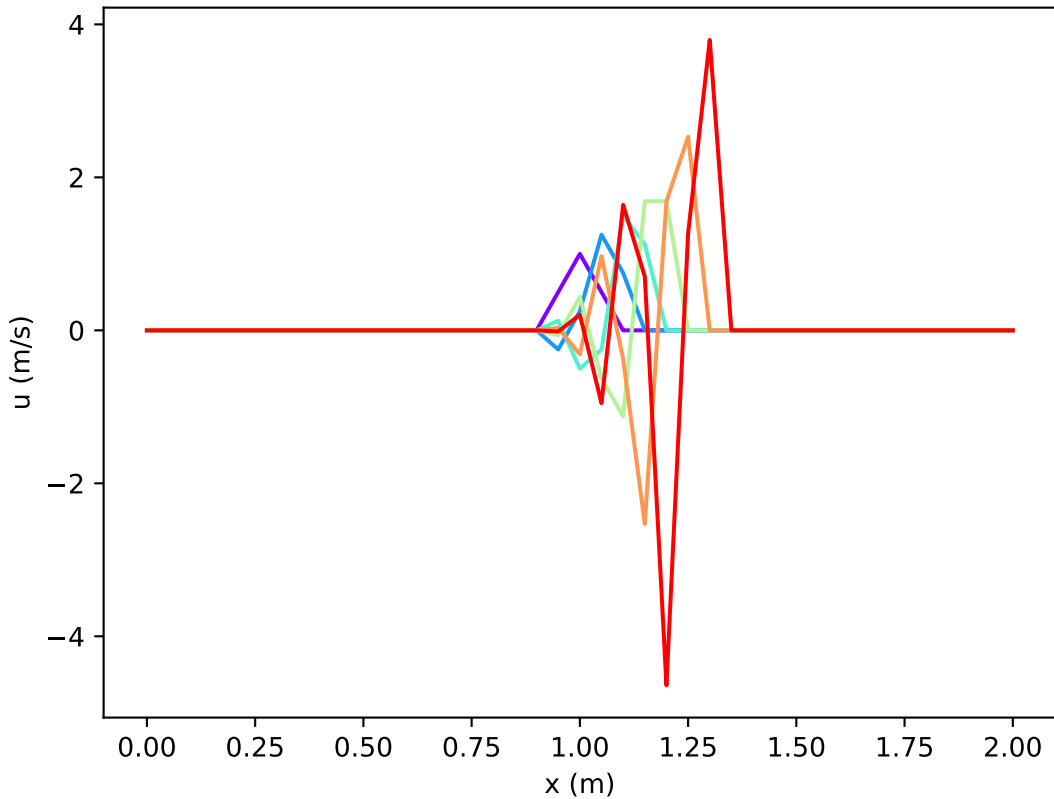
Figure 1: \sigma=1.5 , Backward Differencing in x
