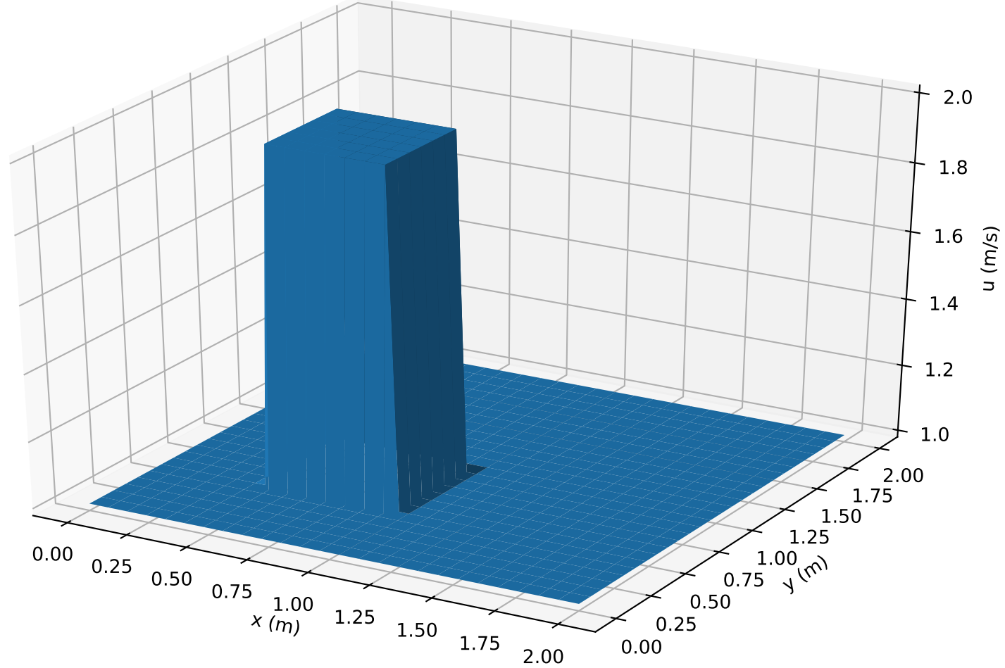
Figure 1: \nu=0.1 , nt=51 , n_x=21 , n_y=21 , t=0\text{sec}
