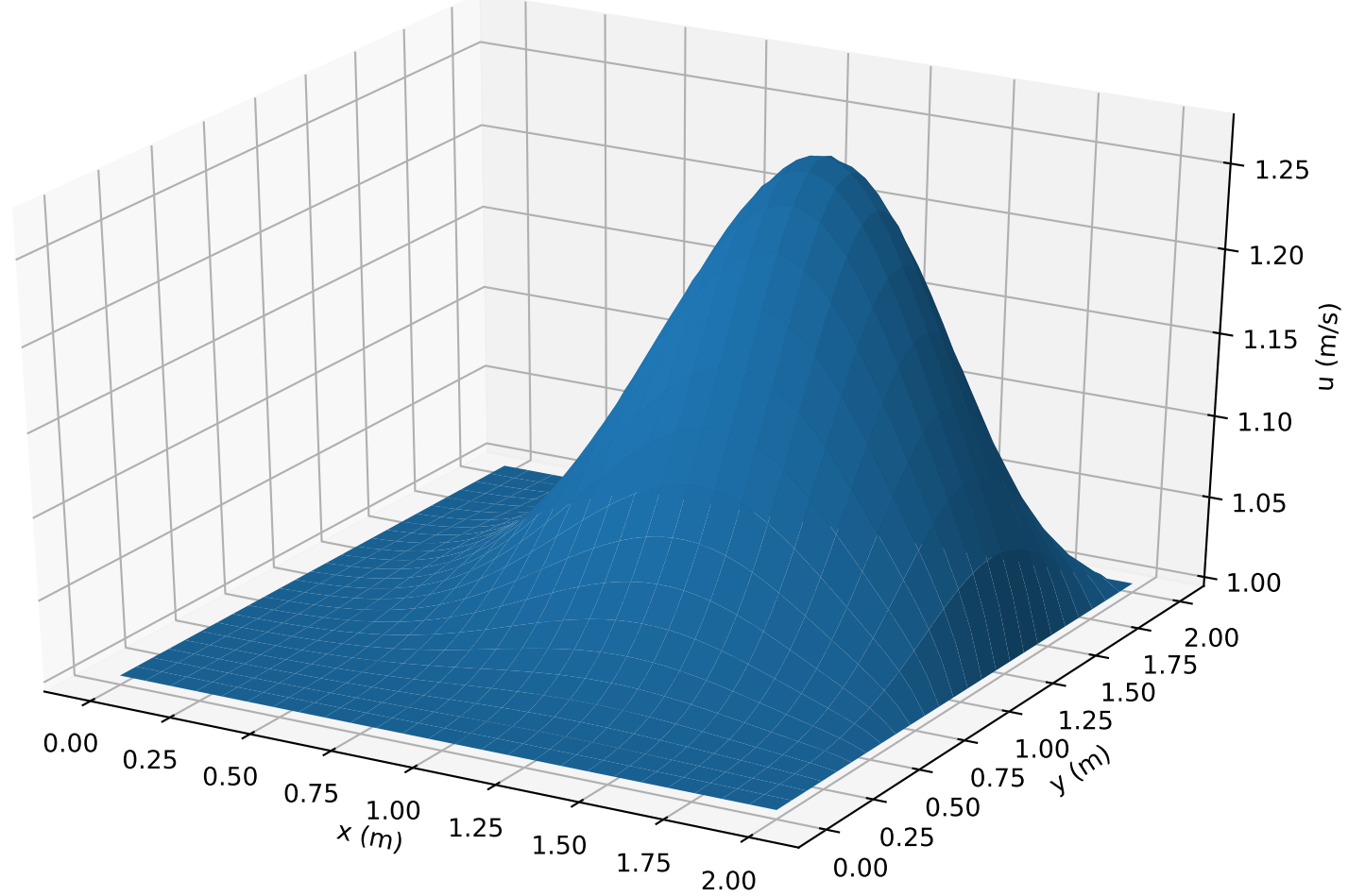
Figure 2: \nu=0.1 , nt=51 , n_x=21 , n_y=21 , t=0.5\text{sec}
