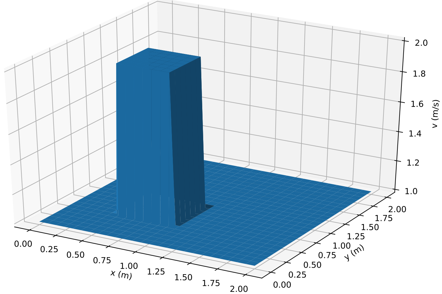
Figure 3: \nu=0.1 , nt=51 , n_x=21 , n_y=21 , t=0\text{sec}
