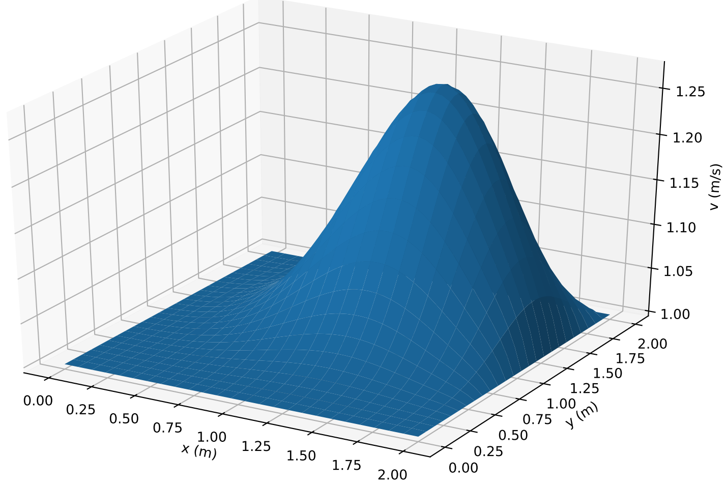
Figure 4: \nu=0.1 , nt=51 , n_x=21 , n_y=21 , t=0.5\text{sec}
