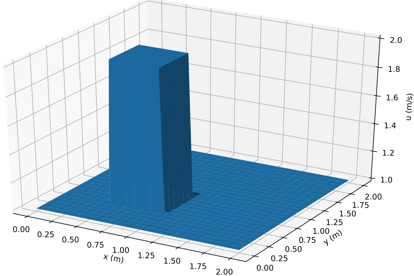
Figure 1: \nu=0.1 , nt=151 , n_x=51 , n_y=51 , t=0\text{sec}
