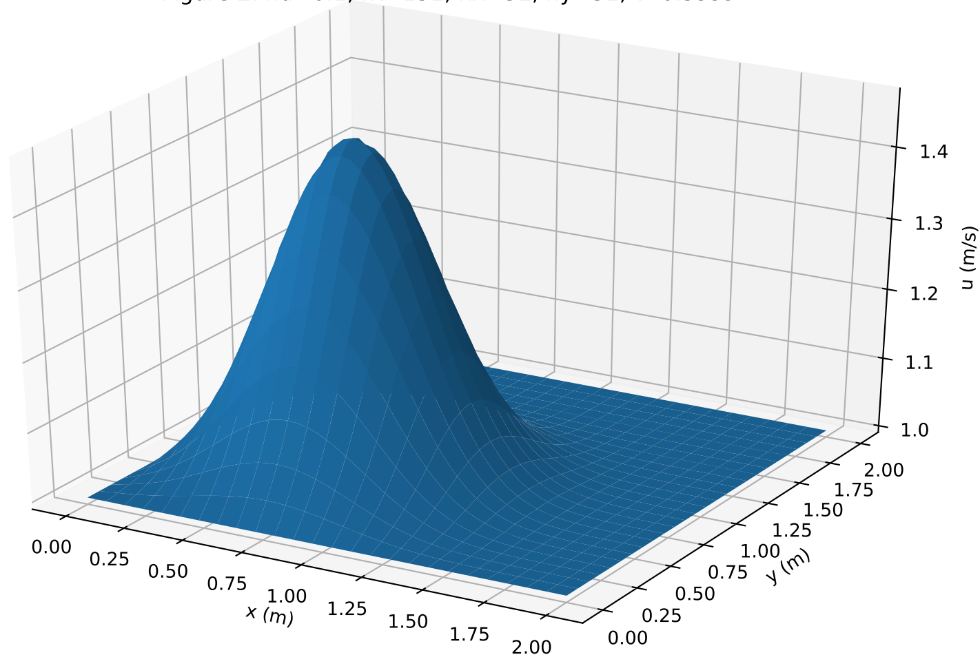
Figure 2: \nu=0.1 , nt=151 , n_x=51 , n_y=51 , t=0.5\text{sec}
