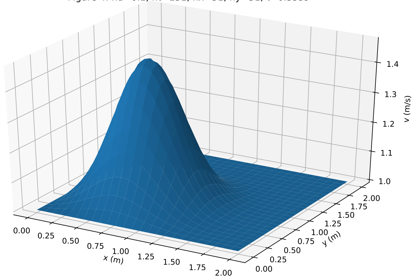
Figure 4: \nu=0.1 , nt=151 , n_x=51 , n_y=51 , t=0.5\text{sec}
